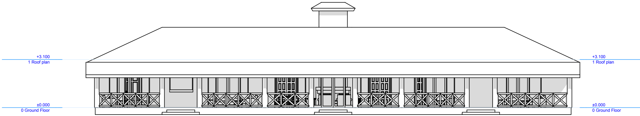
FRONT ELEVATION
