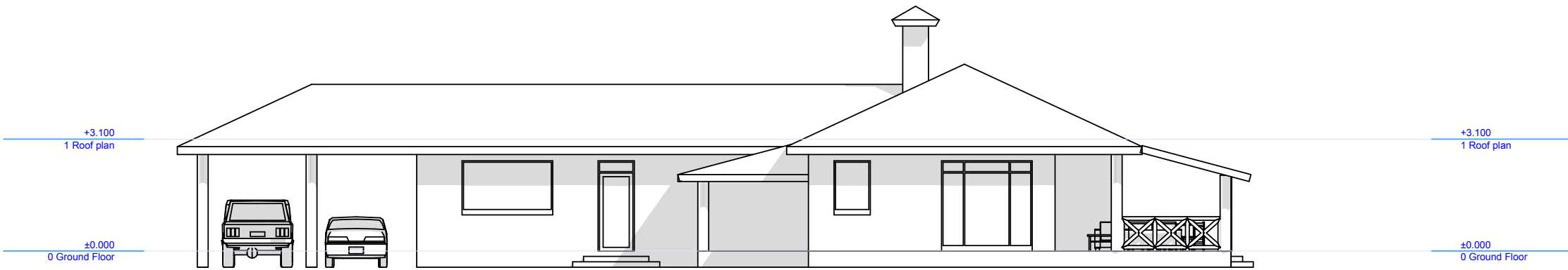
SIDE ELEVATION
